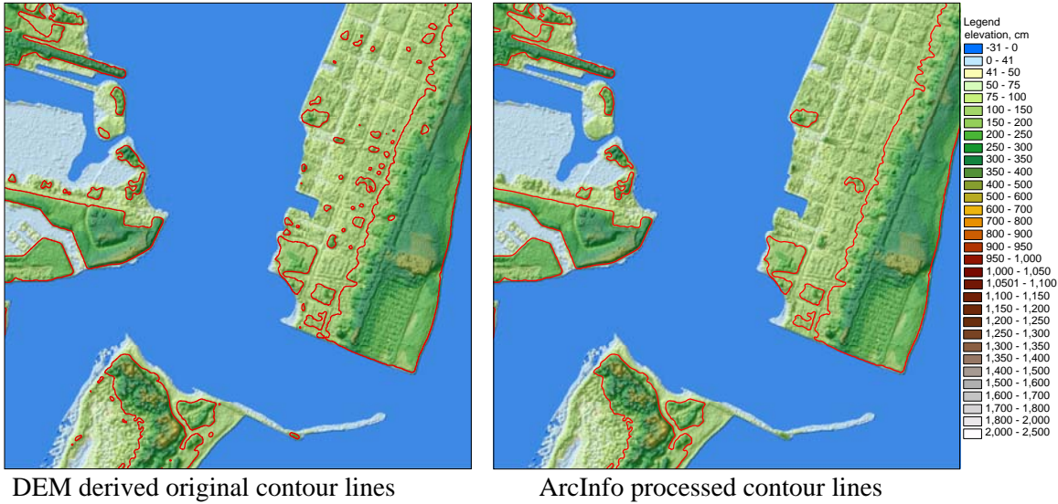
Figure 5. Storm Surge Contour Lines for Category 2 Hurricane
