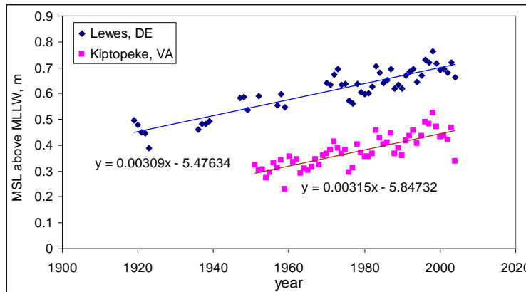
Figure 4. Historic sea level rise trend for Worcester County, MD based on water level observations from Lewes, DE and Kiptopeke, VA tidal stations.
